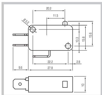
PIN PLUNGER
