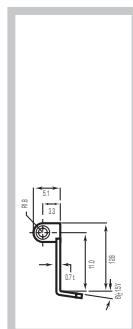
ROLLER LEVER
